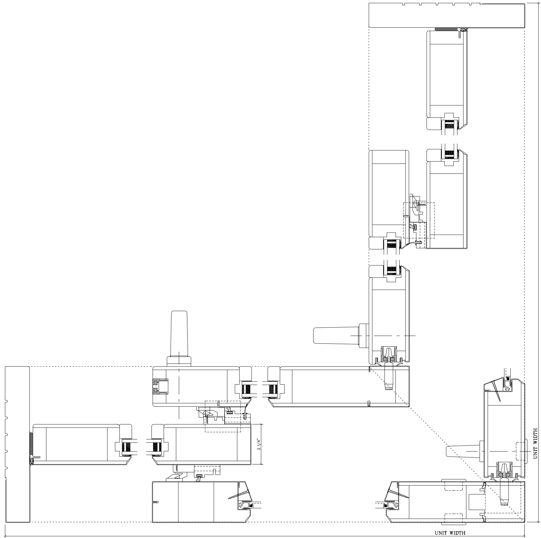
3 LIFT-SLIDE JAMB FULL SCALE
